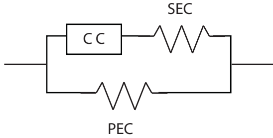
Model [cc + SEC]
